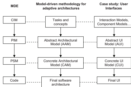
Figure 1. Model-driven methodology
